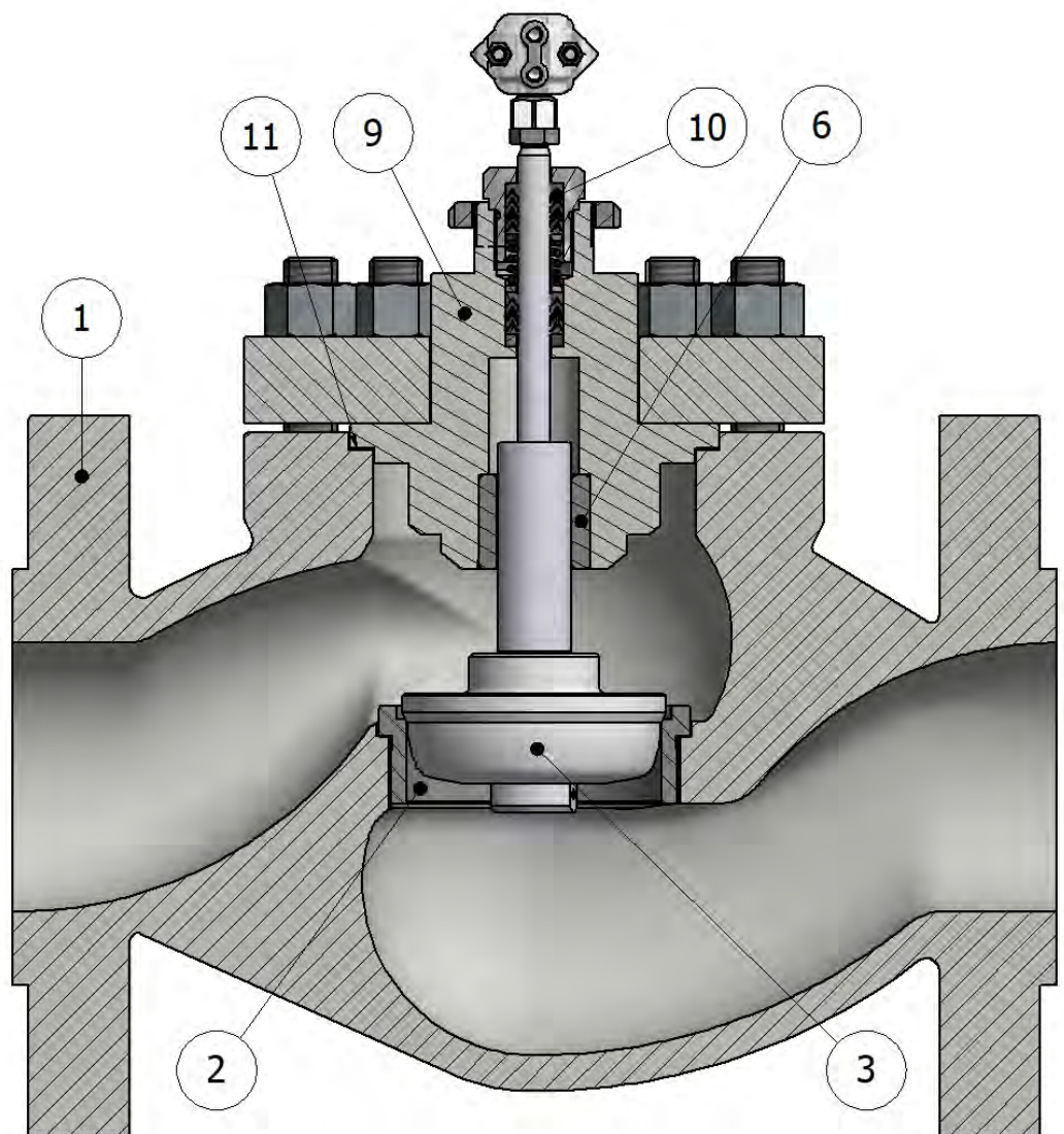
VALVOLA STANDARD
