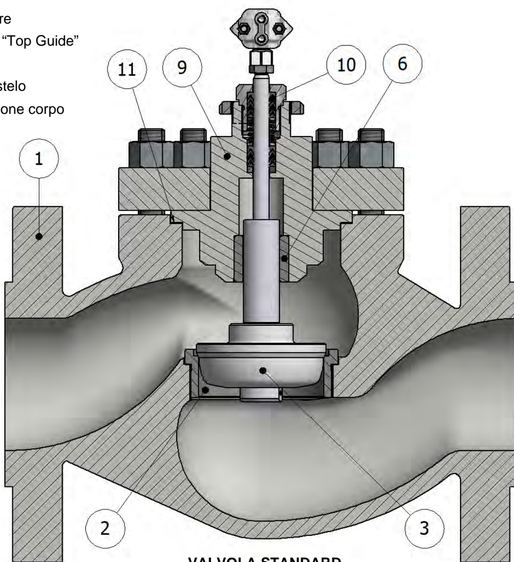
VALVOLA STANDARD
